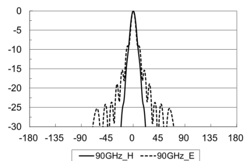
90GHz
